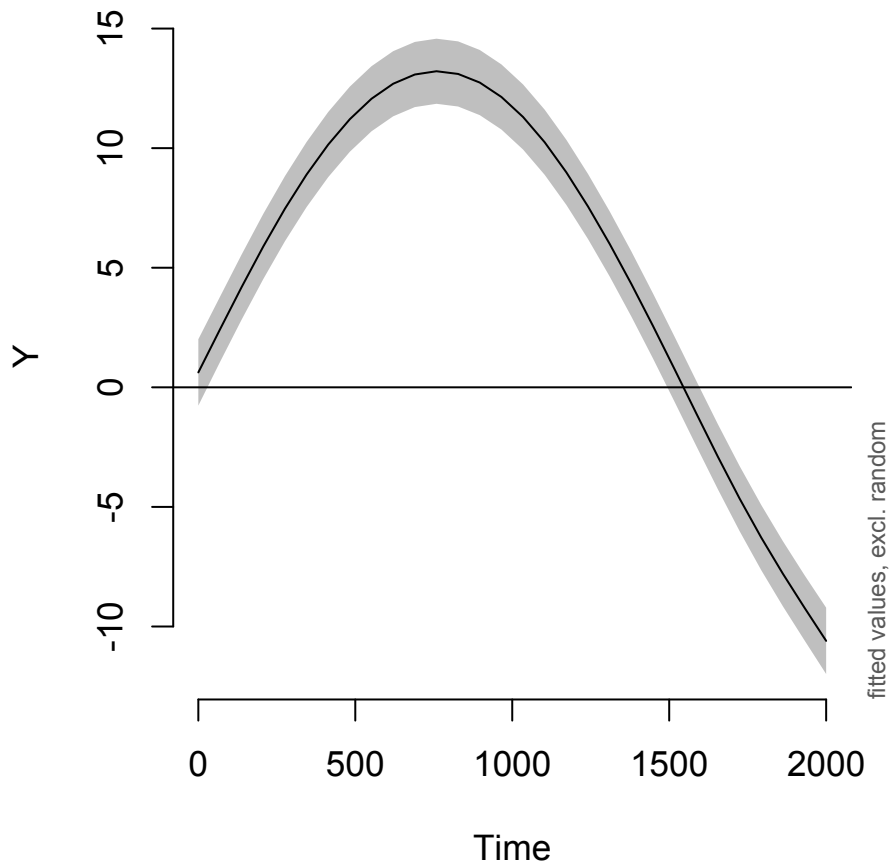
intercept+s(Time):GroupAdults
